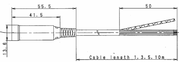
Option: Extension cable (CE22-**)
