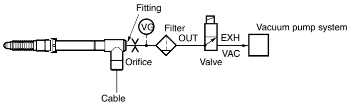
Fig.1 Air-pass system
